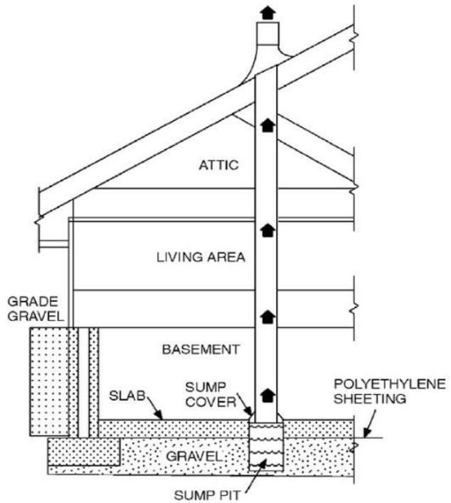
PASSIVE RADON SYSTEM VENTED THROUGH SUMP
