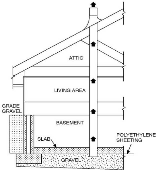
TYPICAL SUBSLLAB DEPRESSURIZATION PASSIVE RADON SYSTEM
