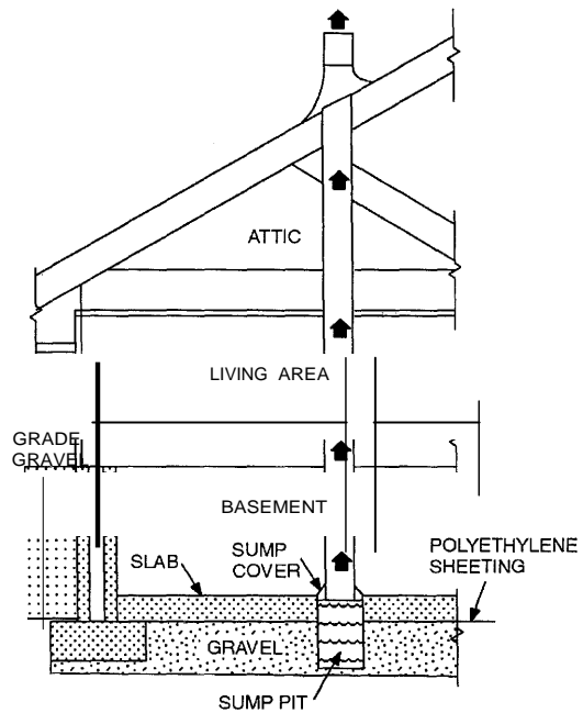
PASSIVE RADON SYSTEM VENTED THROUGH SUMP
