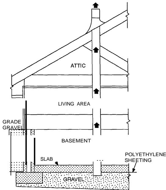
TYPICAL SUB-SLAB DEPRESSURIZATION PASSIVE RADON SYSTEM
