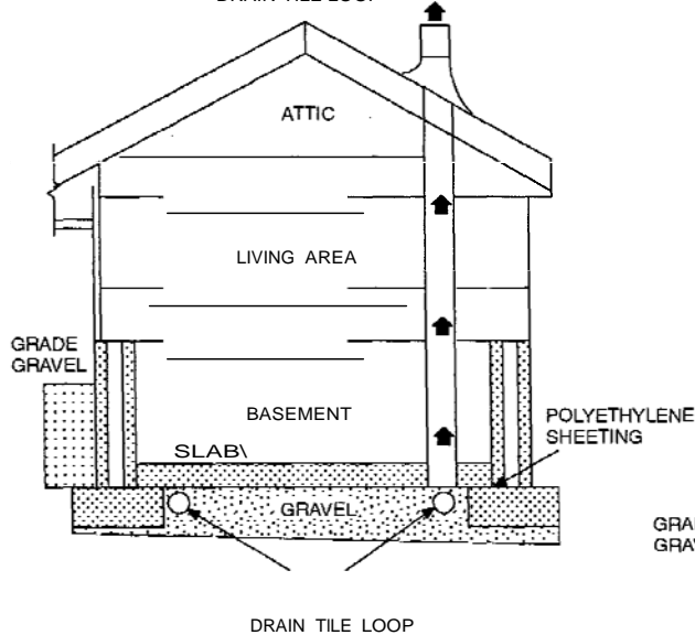
PASSIVE RADON SYSTEM USING DRAIN-TILE LOOP
