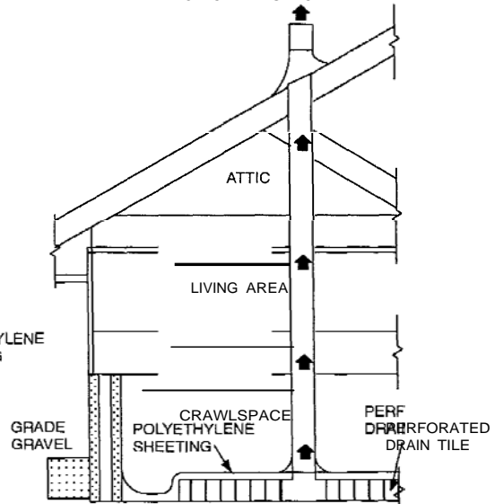
SUB-MEMBRANE DEPRESSURIZATION SYSTEM FOR CRAWL SPACE
